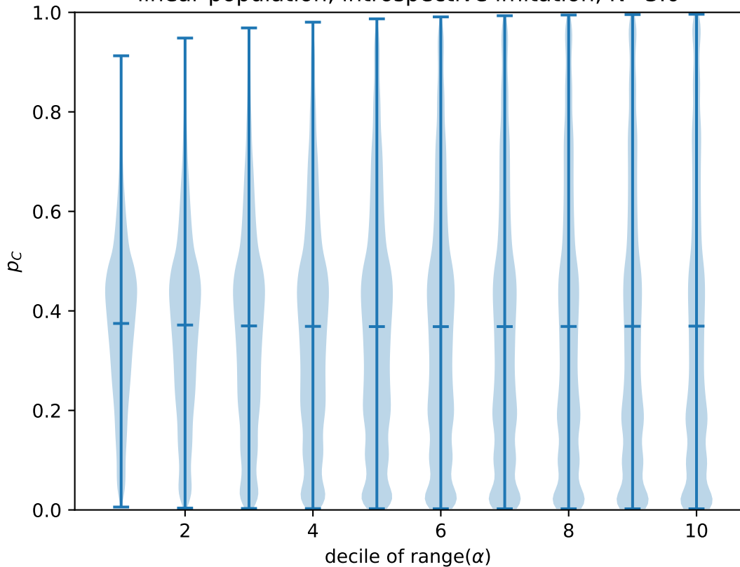
linear population, introspective imitation, N=3.0
